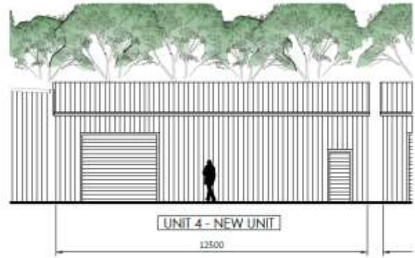
front elevation of new units 4 & 5 scale 1:50 @ A1
